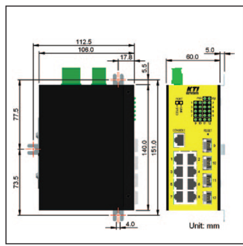
Panel Dimension
