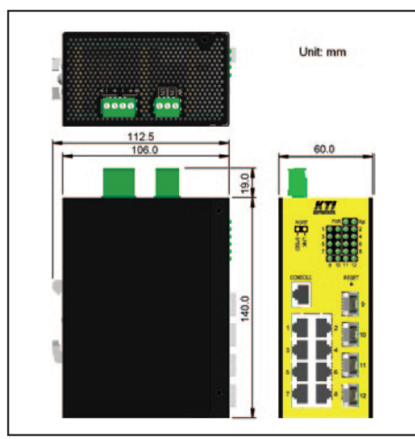
DIN-Rail Dimension
