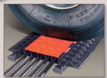
Guard Dog® 5 Channel - protects cable and hose lines up to 1.3 in. outside diameter
